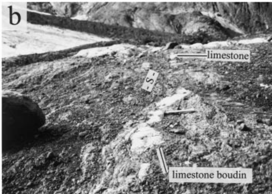
Fig. 7. (a) Geologic map of the toe of Wosnesinski glacier, showing long train of limestone blocks in argillite matrix. Arrow shows view direction of photo (b); (b) photograph of limestone blocks at Wosnesinski glacier.
