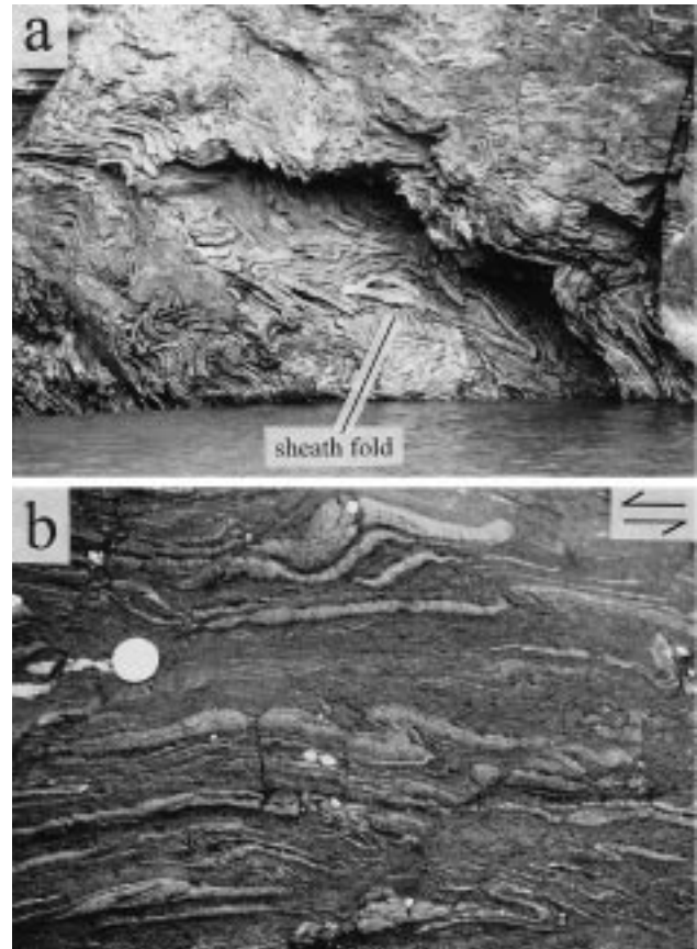
Fig. 5. Folds of layering in mélangé units. (a) Sheath folded chert from Kachemak Bay (fold is approximately 3 m across), (b) folds in graywacke–argillite mélangé.
