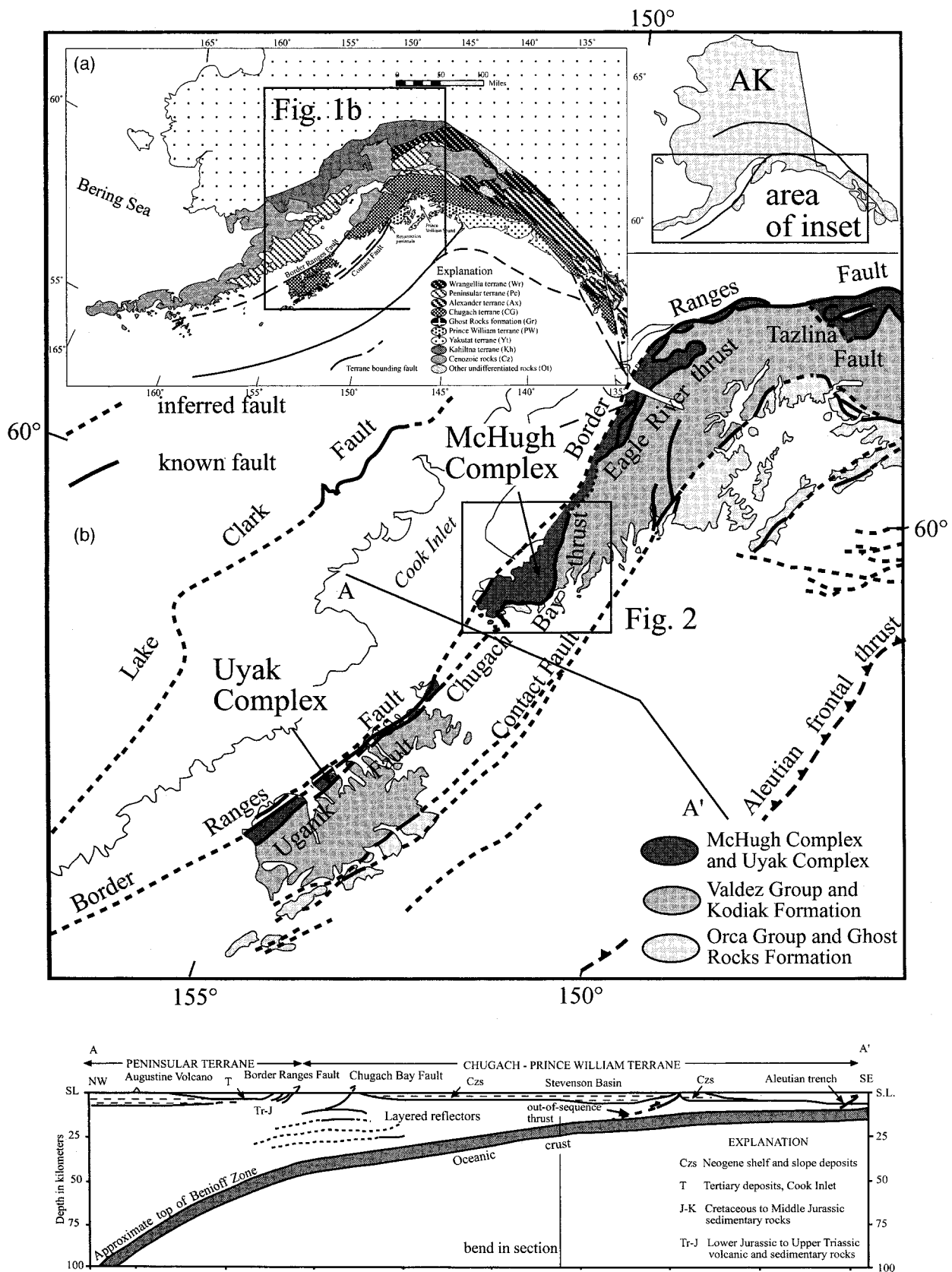
Fig. 1. Map of southern Alaska showing major tectonic elements including the McHugh Complex (and the equivalent Uyak Complex on Kodiak Island). Inset (a) shows tectonic setting of Chugach terrane to the south of the Wrangellia–Alexander–Peninsular superterrane. Detailed map (b) shows the McHugh Complex on the Kenai Peninsula, bounded on the west by the Border Ranges fault, and on the east by the Chugach Bay fault. Box shows location of Fig. 2.
