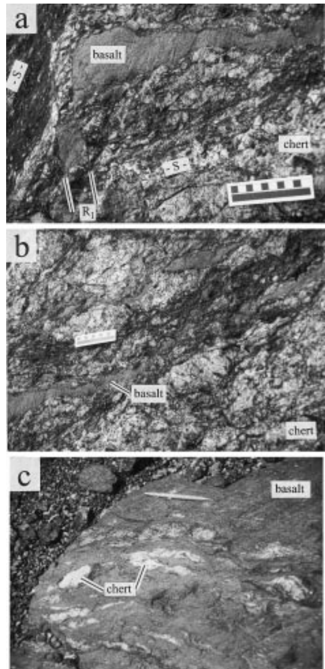
Fig. 11. Basaltic schlieren mixed with chert/argillite mélangé (a and b). Basalt schlieren in (a) is truncated by a shear zone (with C parallel to S ) at a high angle to schlieren elongation, and has associated R_1 shears that further disrupt the basaltic layer, and tend to isolate blocks of basalt within a chert–argillite matrix. (b) Strongly boudinaged end of the basalt schlieren. (c) Chert schlieren mixed with basaltic mélangé.
